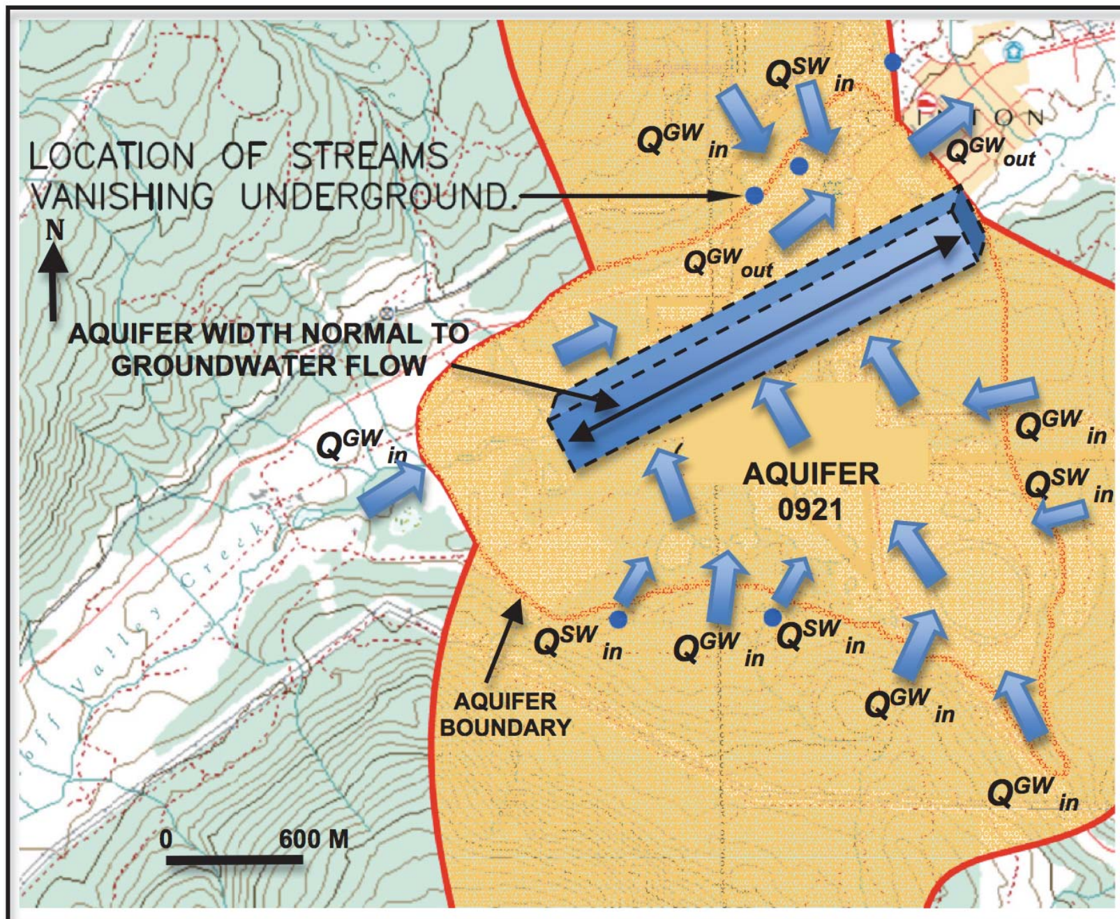
Figure 9. Application of Darcy's Law to estimate groundwater outflow component in lower reaches of aquifer showing inferred groundwater flow directions. Base drawing from EHD Consulting Ltd (2018).
